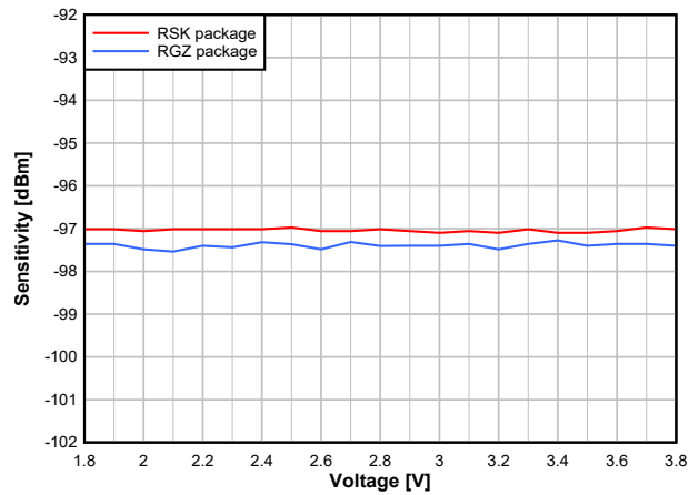
Figure 7-22. Sensitivity vs. Supply Voltage (VDDS) (BLE 1Mbps, 2.44GHz)
