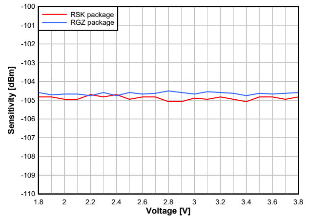
Figure 7-23. Sensitivity vs. Supply Voltage (VDDS) (250kbps, 2.44GHz)
