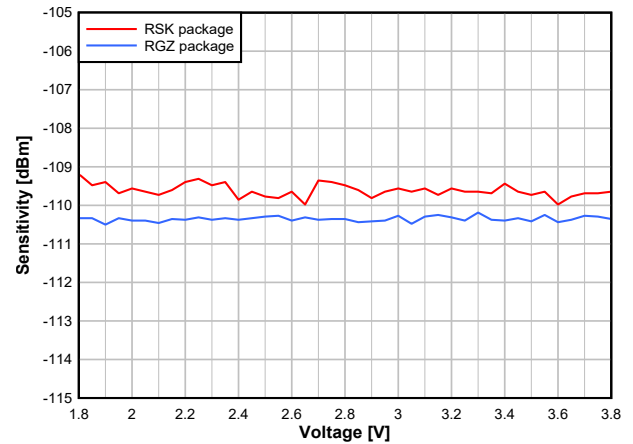
Figure 7-21. Sensitivity vs. Supply Voltage (VDDS) (50kbps, 868.3MHz)
