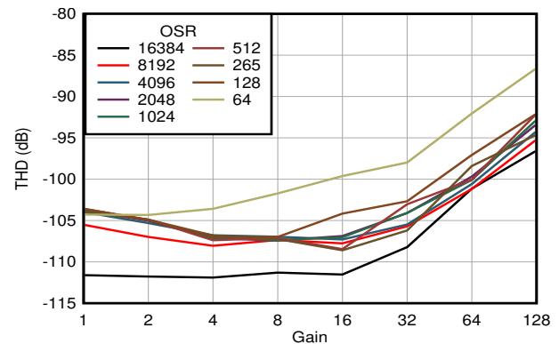
FIG 6-27. THD vs Gain
